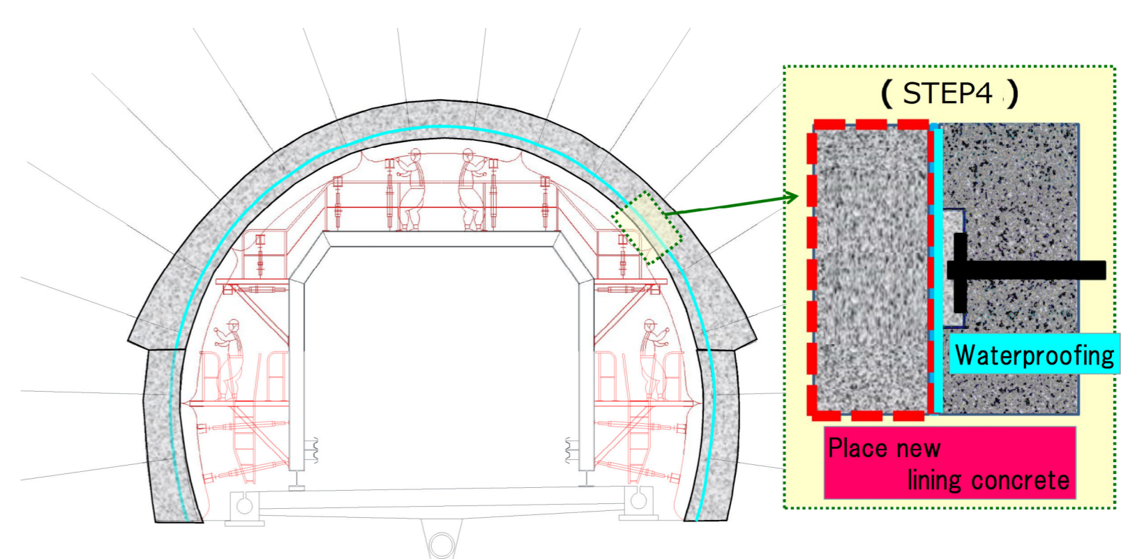
STEP4 Lining concrete placement
