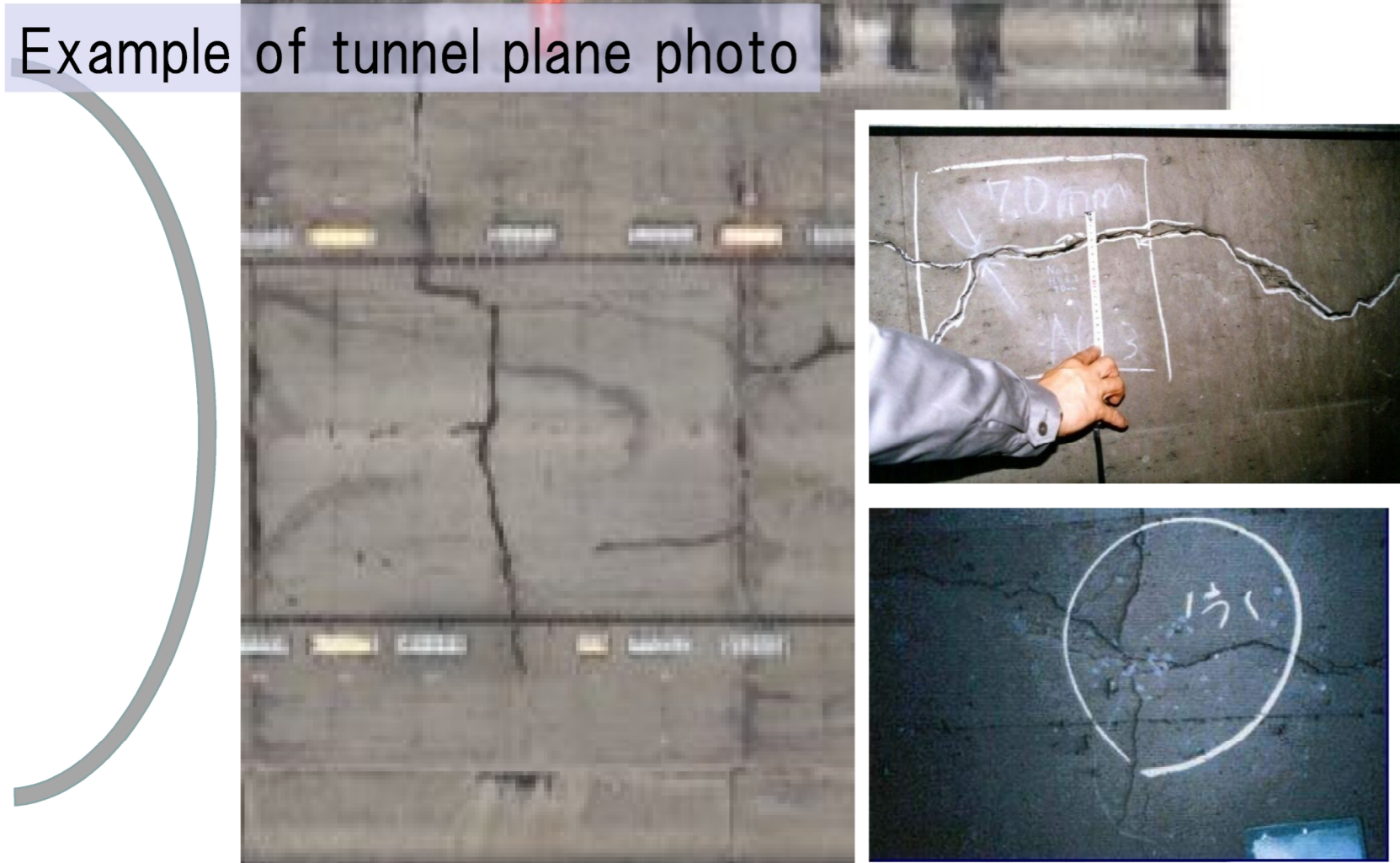
Cracks in lining concrete
