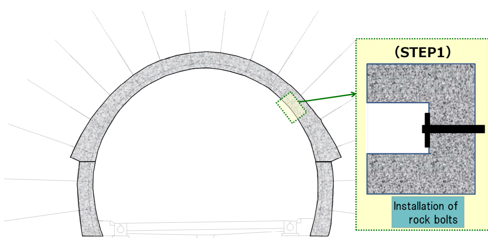
STEP1 Reinforce the tunnel with rock bolts before cutting the existing lining concrete.
