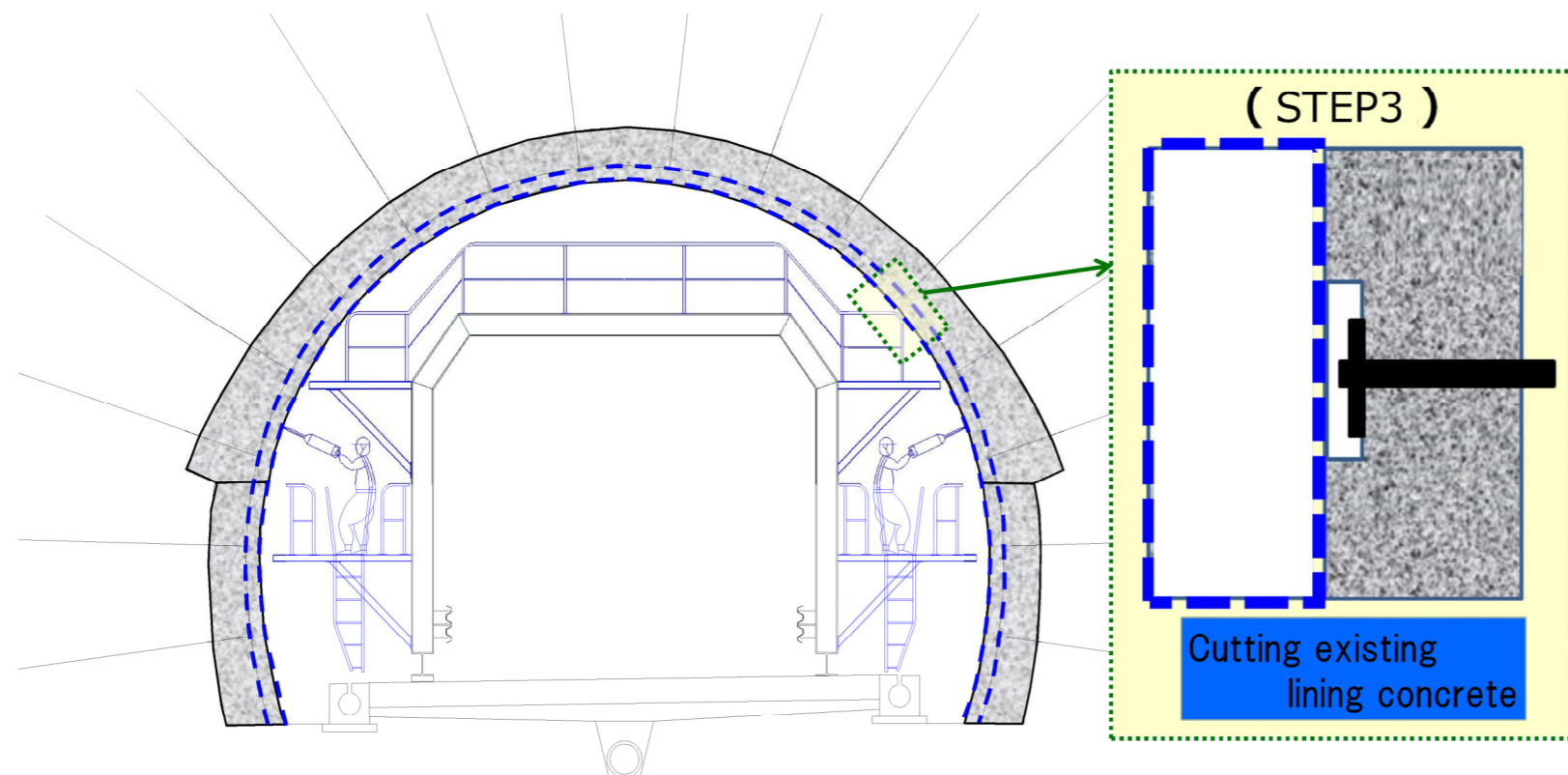
STEP3 Cutting lining concrete
